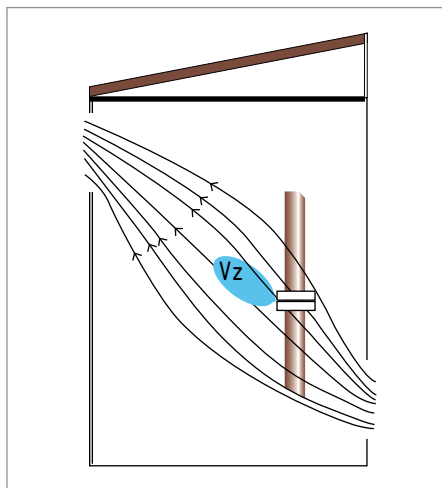
Figure 16: High ventilation
